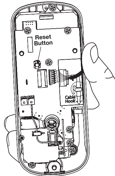
Interior Escutcheon
